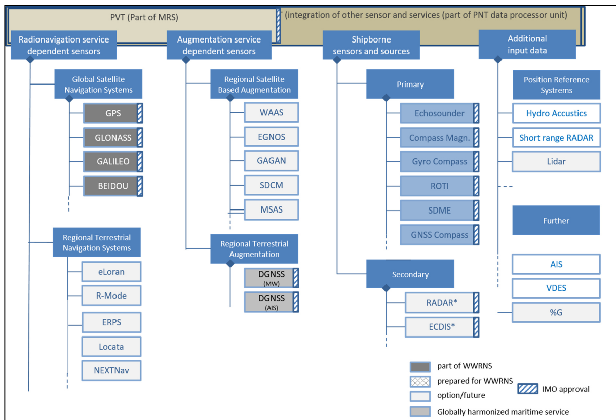
Figure 5: Sensors Services and sources to Provide PNT on board vessels 2
