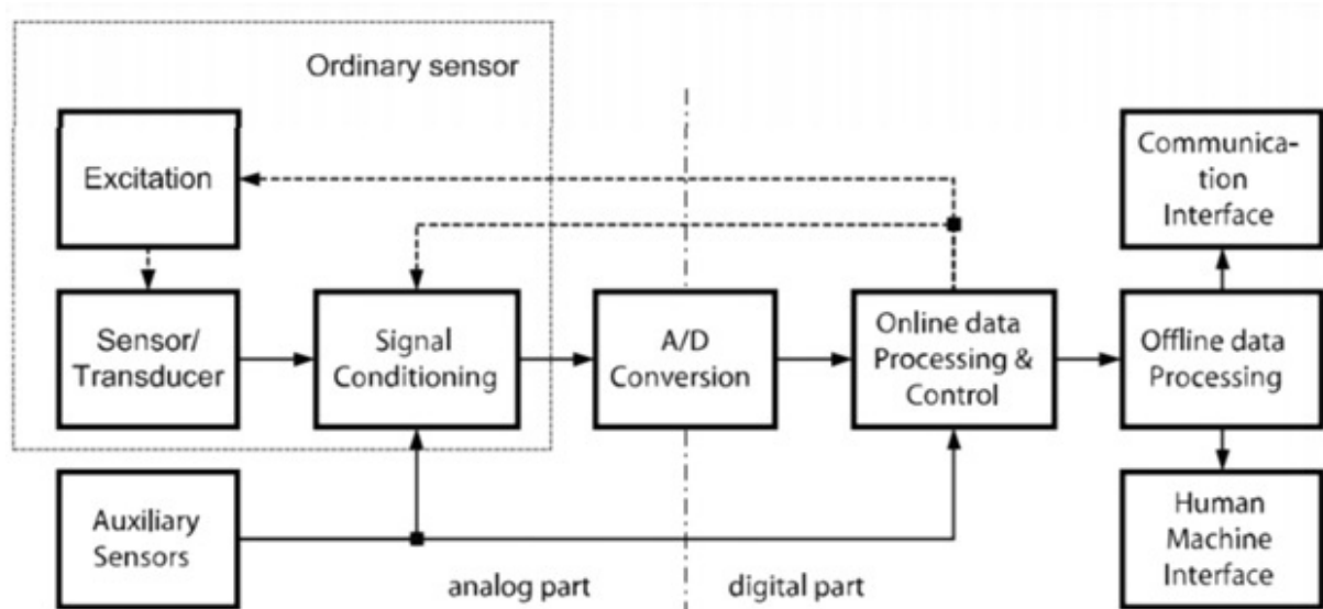
Figure 2: Intelligent sensor structure (Automationforum.co)
