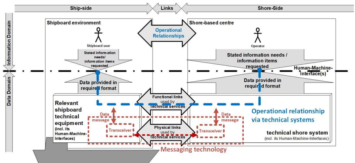
Figure 8: Voice and datalink communications implied by overarching e-navigation architecture
