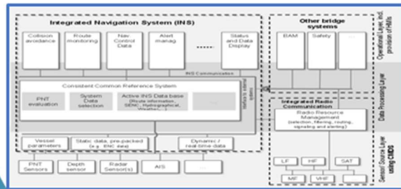
IWT Fairway & Navigation Standardised Shipboard System Architecture (Inland-SSSA)
