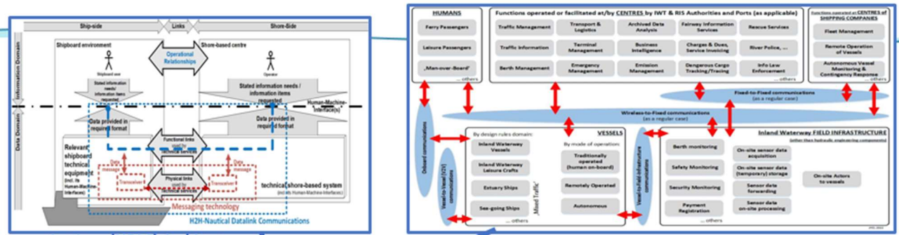
IWT Fairway & Navigation System Interconnections Architecture (ISIA)
