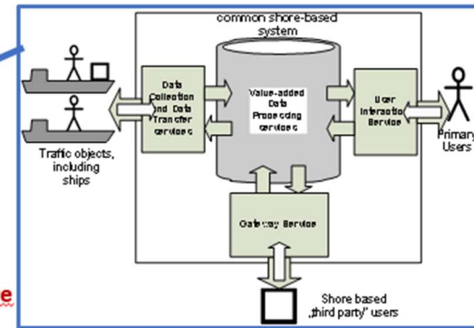
IWT Fairway & Navigation Common Shore System Architecture (Inland-CSSA)
