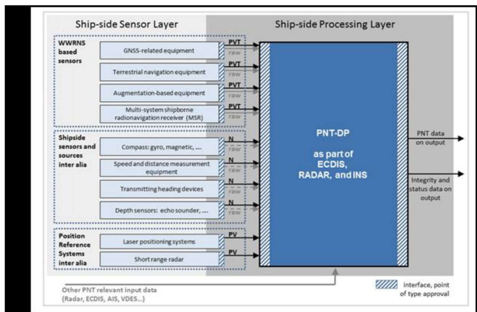
Figure 26: Shipborne PNT Data Processing (PNT-DP) integrated as software into INS, ECDIS, or Radar
